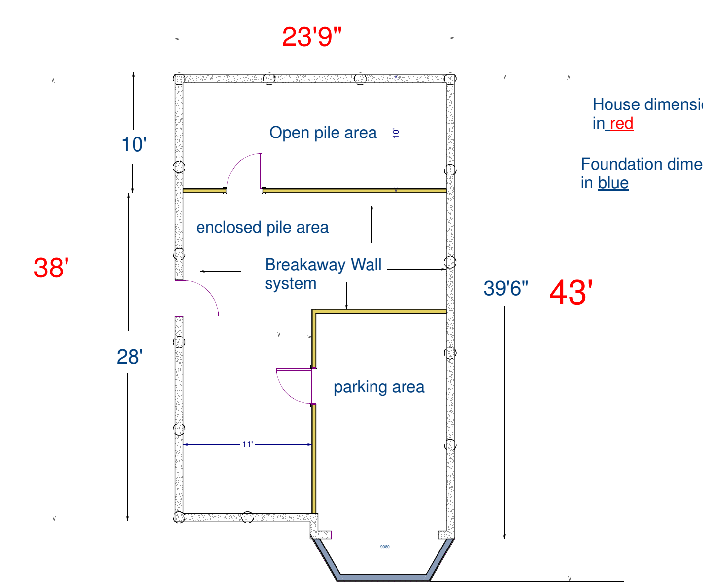
Cantilevered house section above
