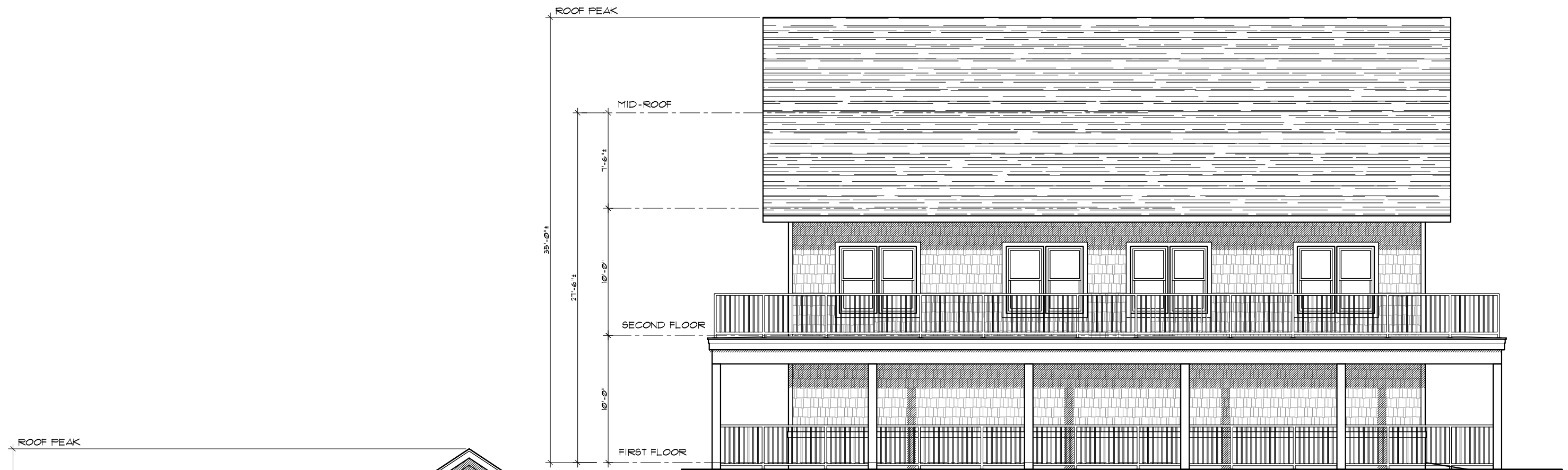
WEST ELEVATION
