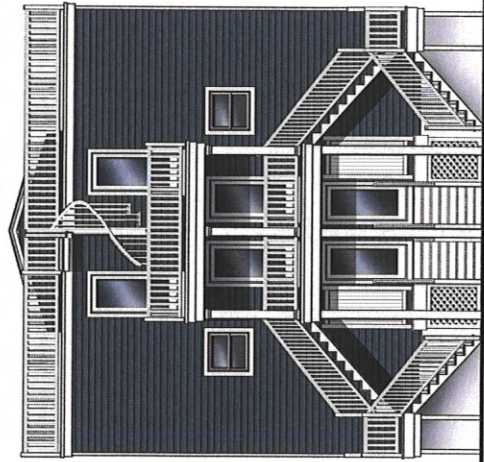
Rear Elevation
